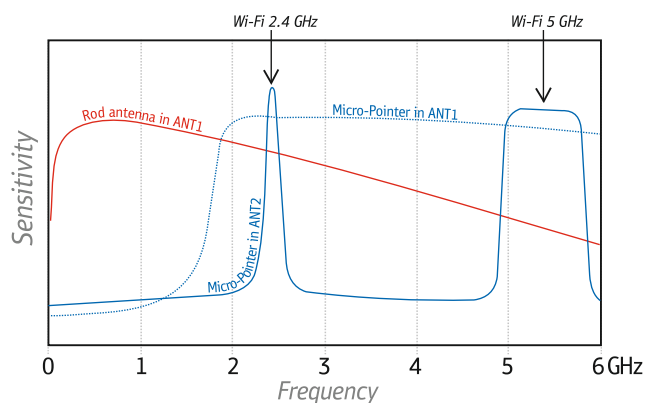
Sensitivity graph of the Protect 1206i
